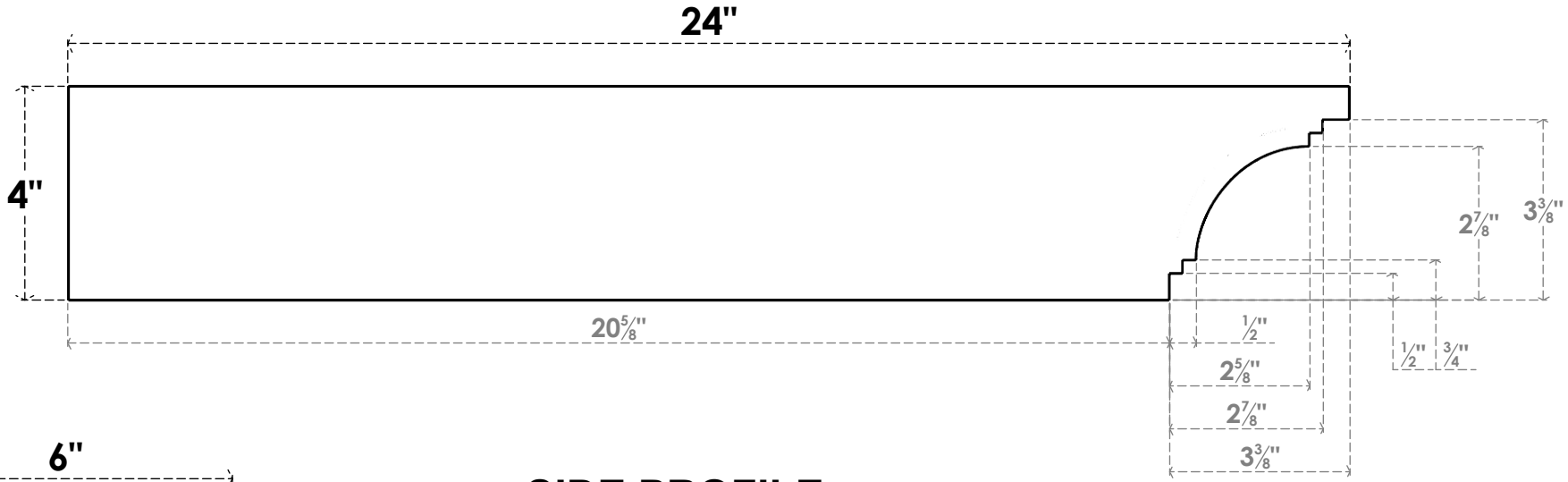
SIDE PROFILE
